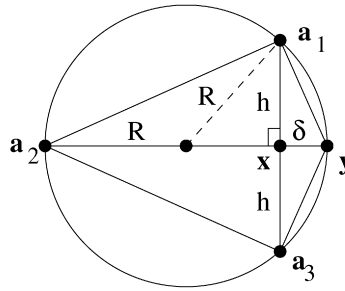
Fig. 6. Lines in proof of Theorem 5.
