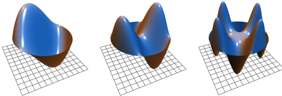
Fig. 8. Hermite mean value interpolants.
