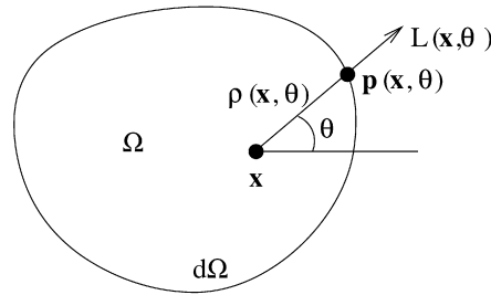
Fig. 1. A convex domain.
