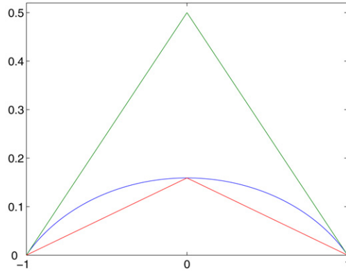
Fig. 5. Upper and lower bounds for the unit disk.
