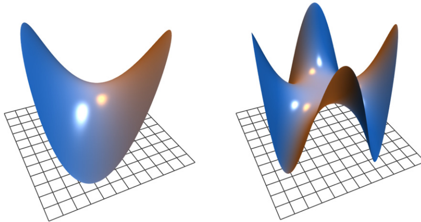
Fig. 2. Mean value interpolants.
