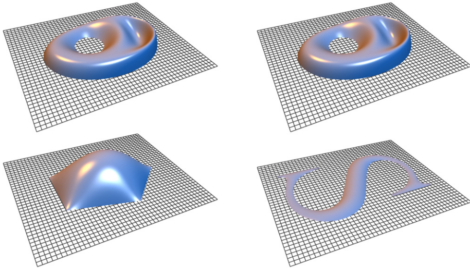
Fig. 11. Numerical solution using bicubic web-splines.
