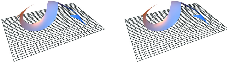
Fig. 12. Solving inhomogeneous problems.
