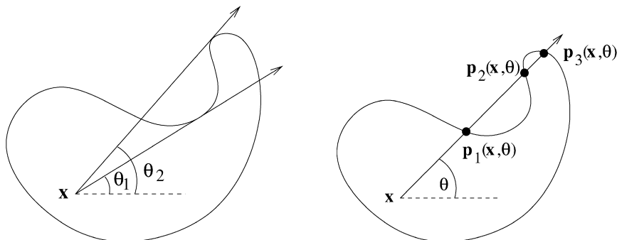
Fig. 3. (left) Example with two non-transversal angles and (right) an angle with three intersections.
