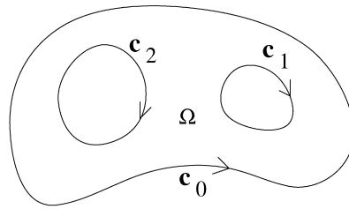
Fig. 9. Multiply connected domain.
