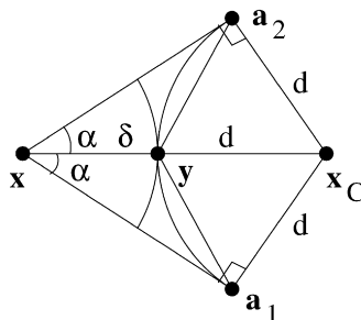
Fig. 4. Lines in proof of Theorem 3.
