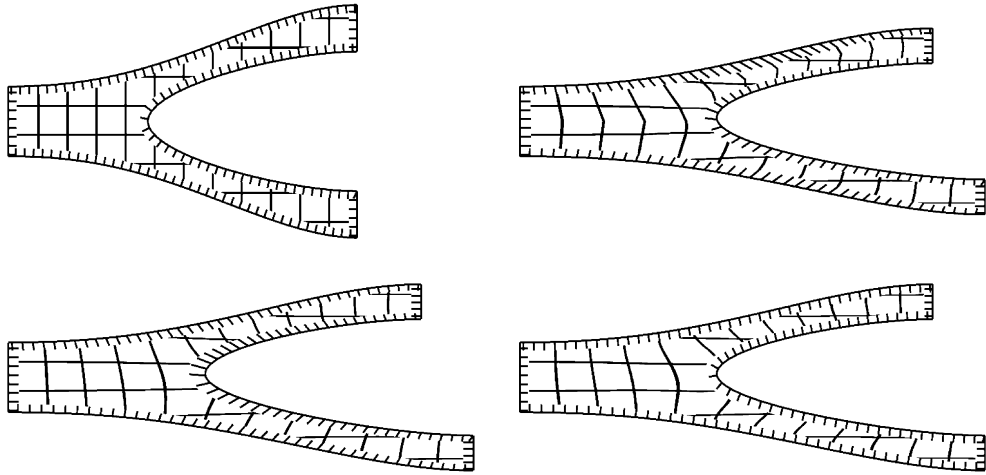
Fig. 10. A bifurcation prototype is mapped to a deformed bifurcation using different transfinite interpolants.
