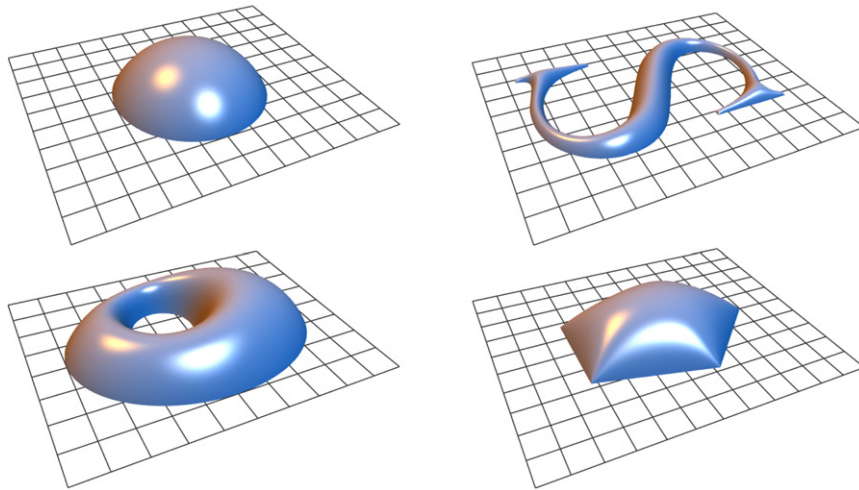
Fig. 7. The weight function \psi on various domains.
